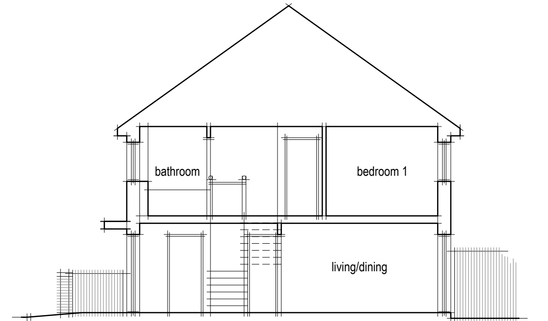
indicative section
