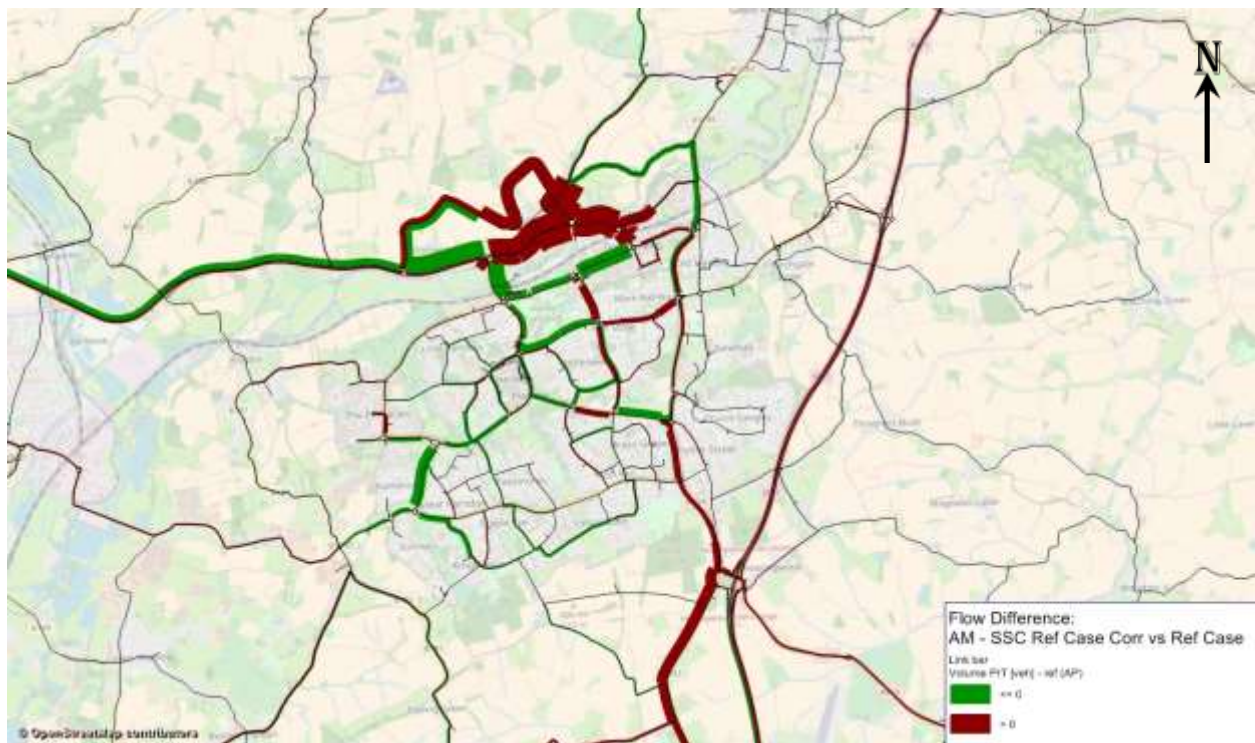
Figure 4-5: Flow Differences – Reference Case with SSC and Bus Lane v. Reference Case (AM peak) S21 vs E1
