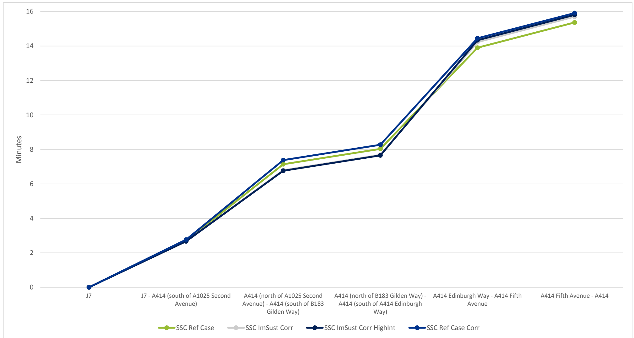
Figure 5-9: Comparison of journey times for J7 to A414 via A414, A414 Edinburgh Way, SSC, and Eastwick Road route
