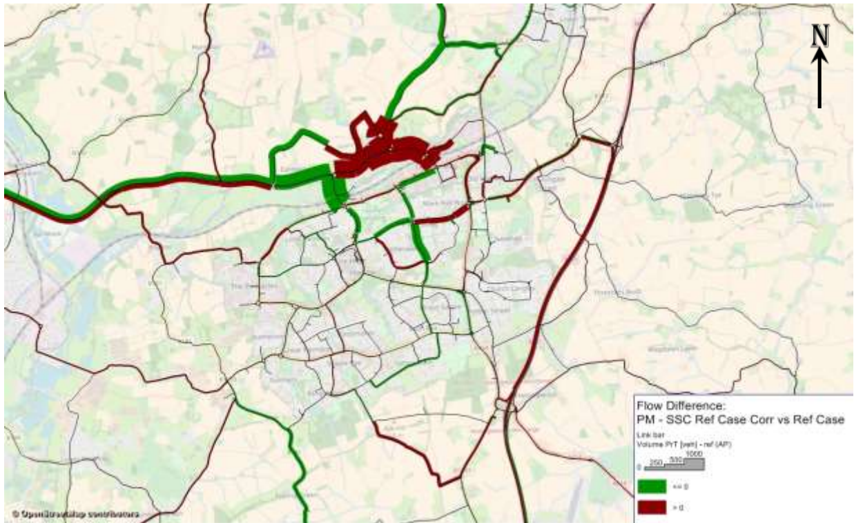
Figure 4-6: Flow Differences – Reference Case with SSC and Bus Lane v. Reference Case (PM peak) S21 vs E1
