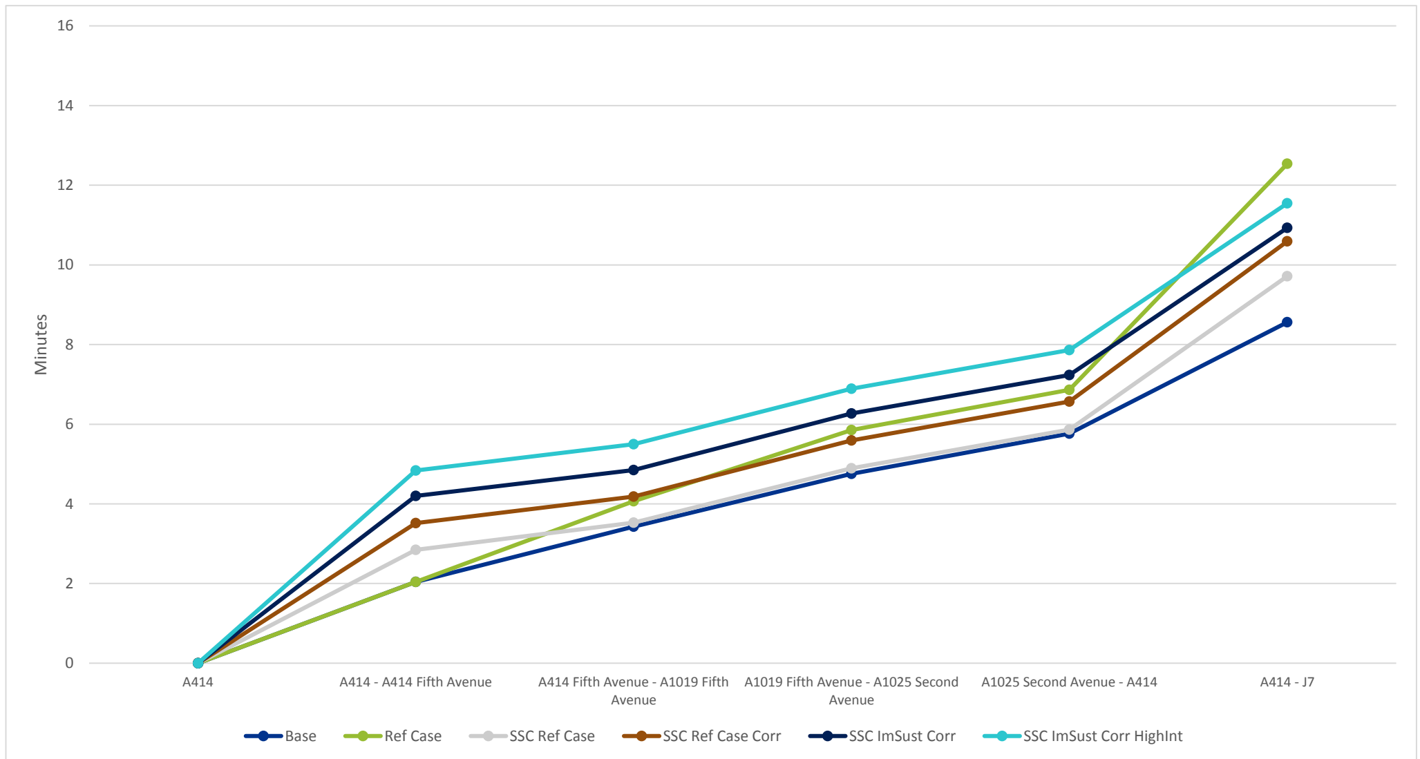
Figure 5-5: Comparison of journey times for A414 to J7 via A414 Fifth Avenue, A1019 Fifth Avenue, A1025 Second Avenue and A414 route
