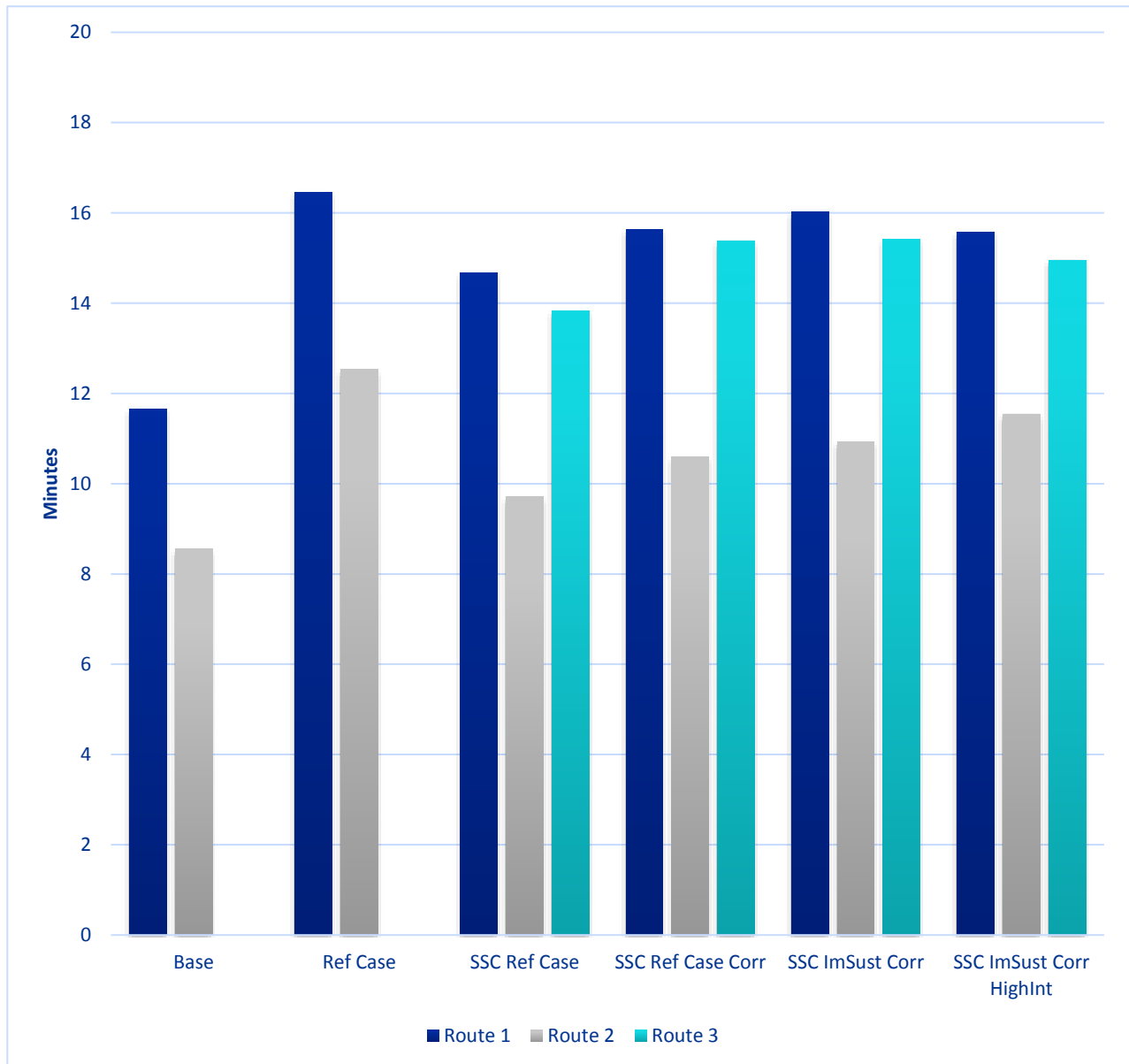
Figure 5-17: Southbound – Travel Time Comparison of the Three Routes from A414 to J7
