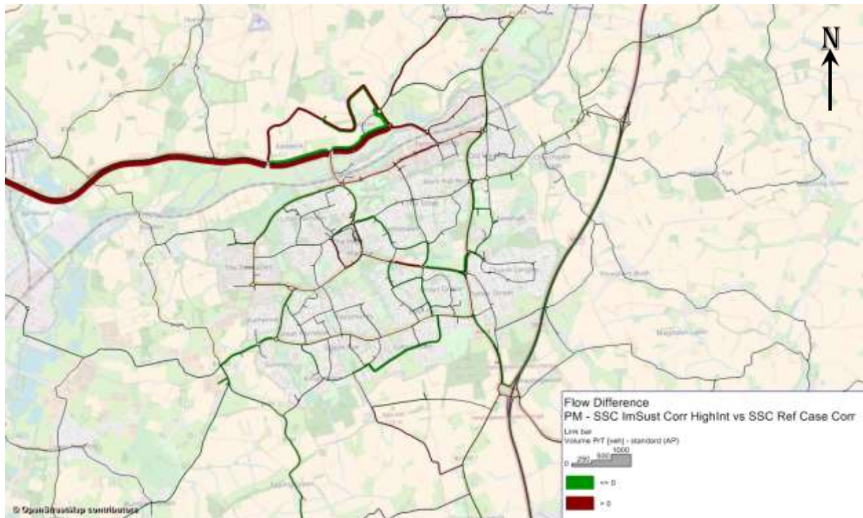
Figure 4-10: Flow Differences – Intermediate Sustainability Scenario with Higher Internalisation v. Reference Case (with SSC and Bus Lane, PM peak) S21LB vs S21
