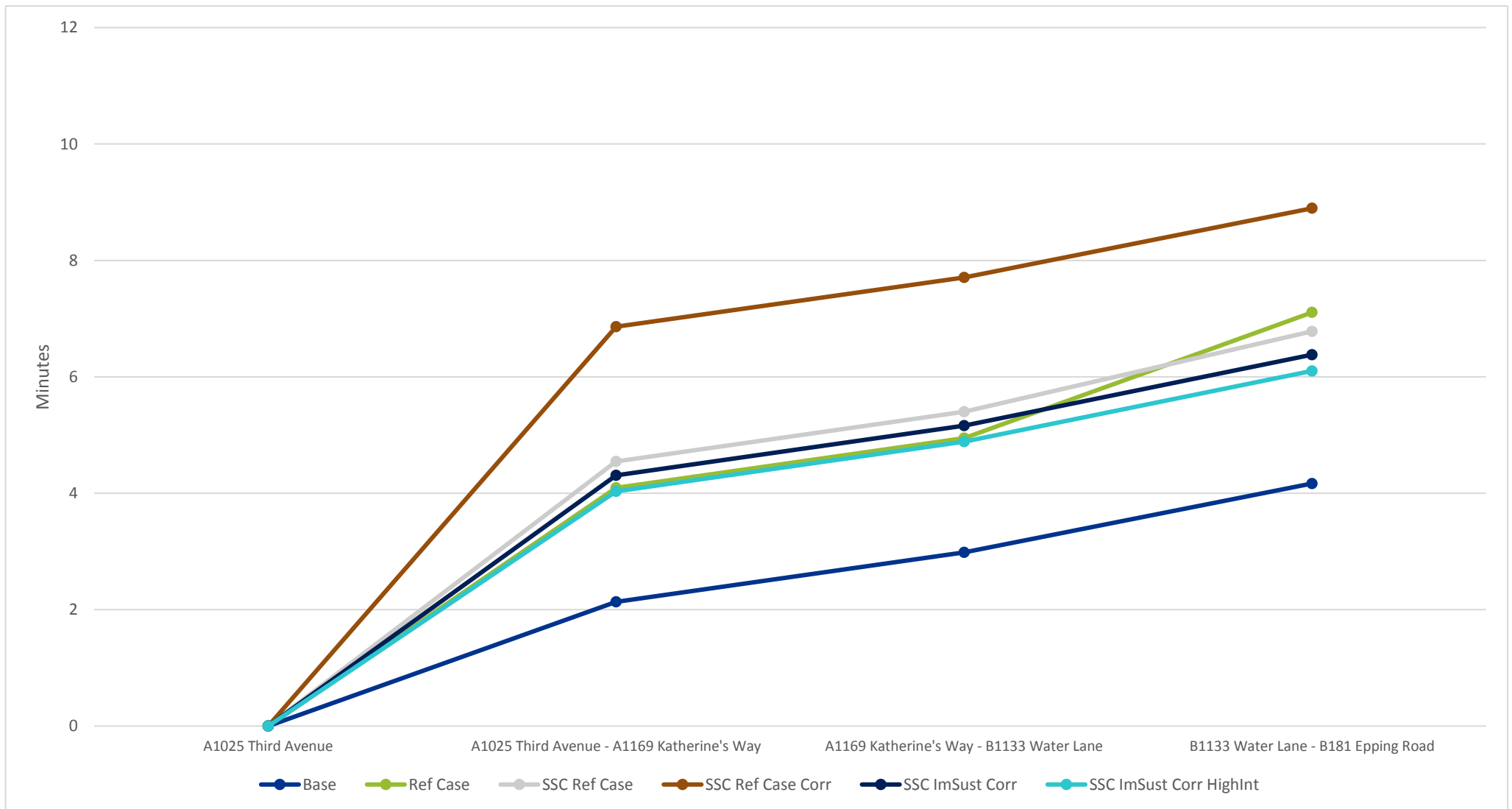
Figure 5-14: Comparison of journey times for A1025 Third Avenue to B1133 Water Lane via A1169 Katherine's Way route
