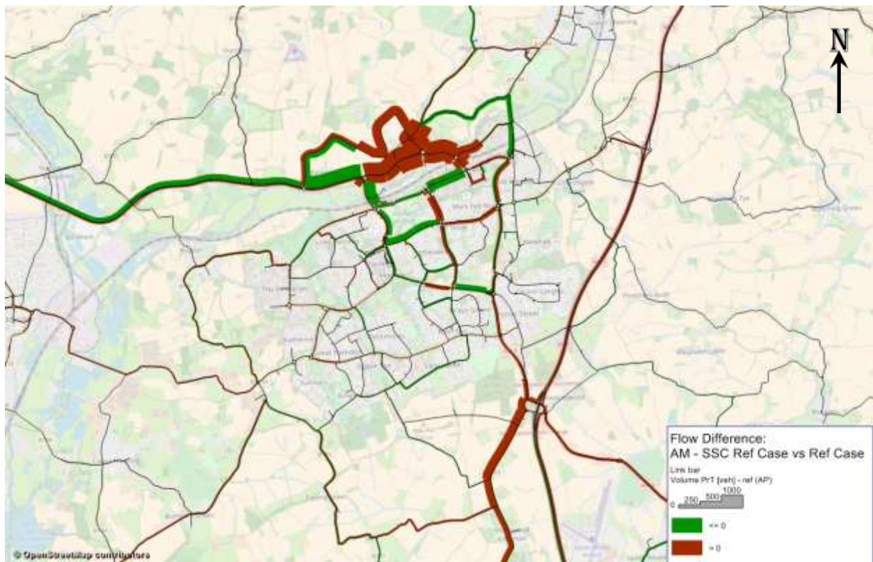
Figure 4-2: Flow Differences Reference Case with SSC v. – Reference Case (AM peak) S1 vs E1
