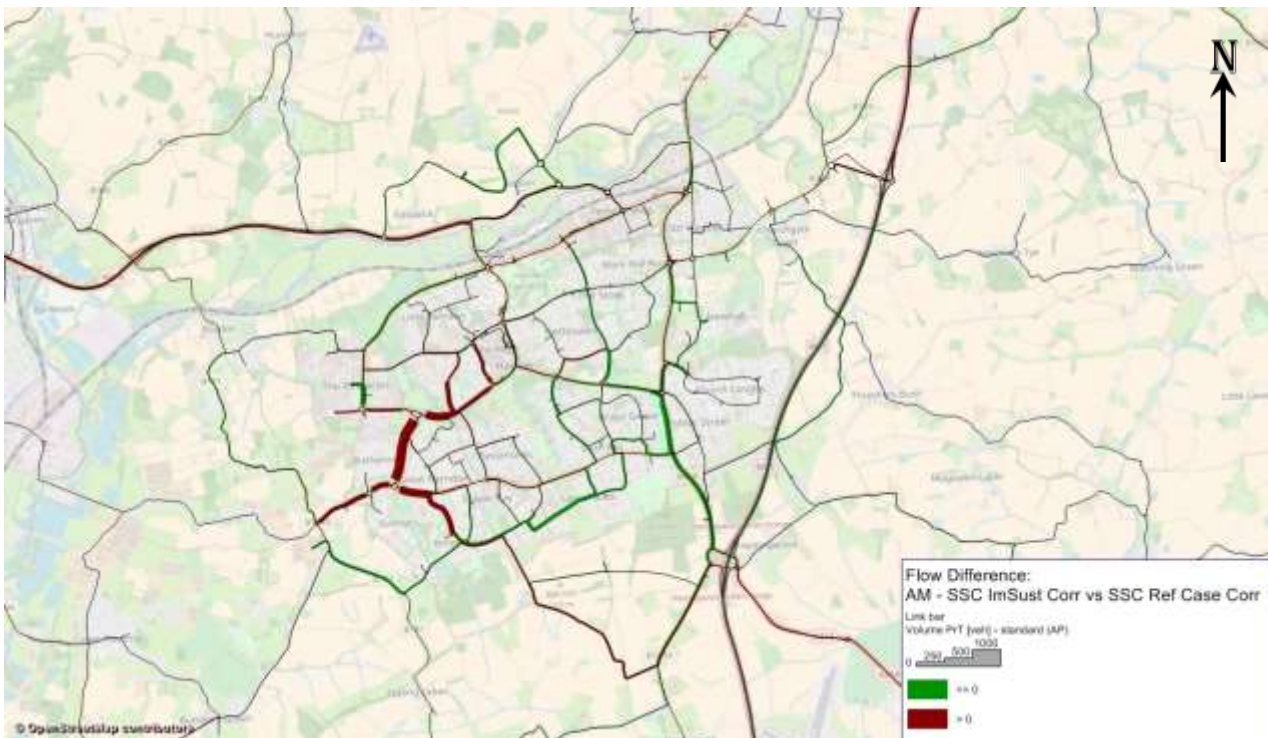
Figure 4-7: Flow Differences – Intermediate Sustainability Scenario v. Reference Case (with SSC and Bus Lane, AM peak) S21B vs S21
