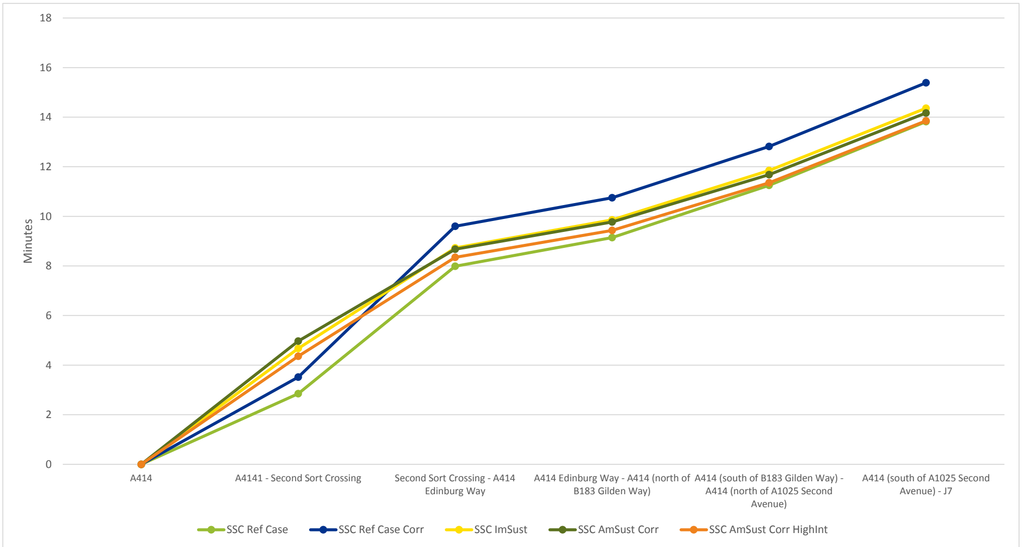
Figure 15: Comparison of journey times for A414 to J7 via Eastwick Road, Second Stort Crossing, A414 Edinburgh Way, and A414 route
