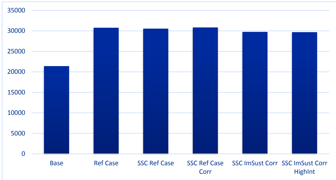
Figure Error! No text of specified style in document.-27: PM – Total Number of Trips (veh)
