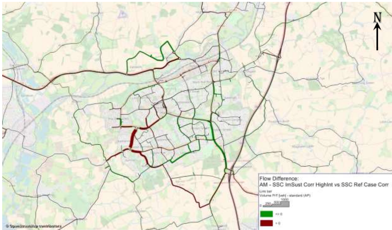
Figure 4-9: Flow Differences – Intermediate Sustainability Scenario with Higher Internalisation v. Reference Case (with SSC and Bus Lane, AM peak) S21LB vs S21
